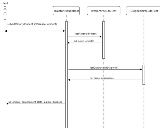
Fig. 3. Sequence diagram of the case "order creation"
